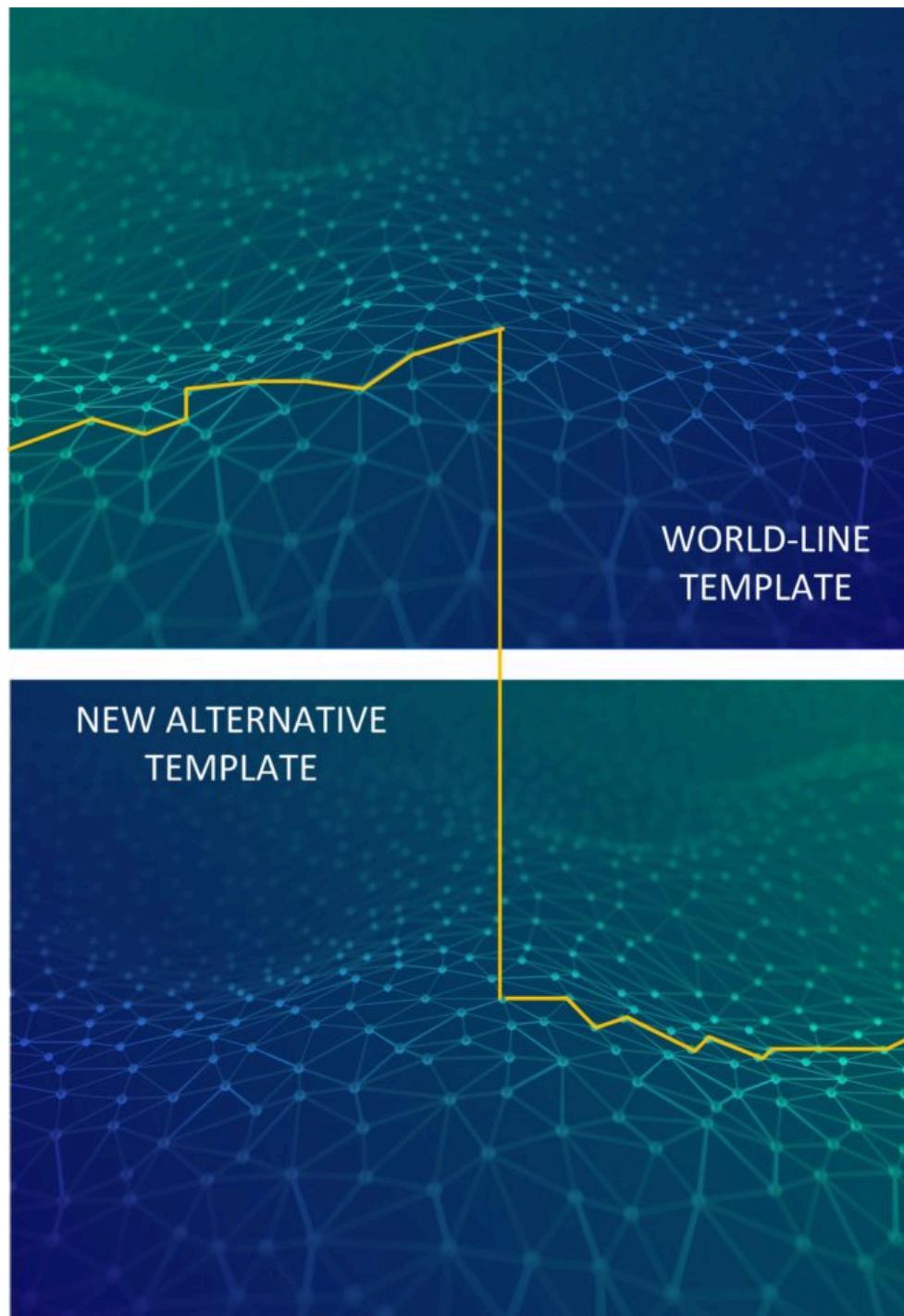
World-Line Slide
